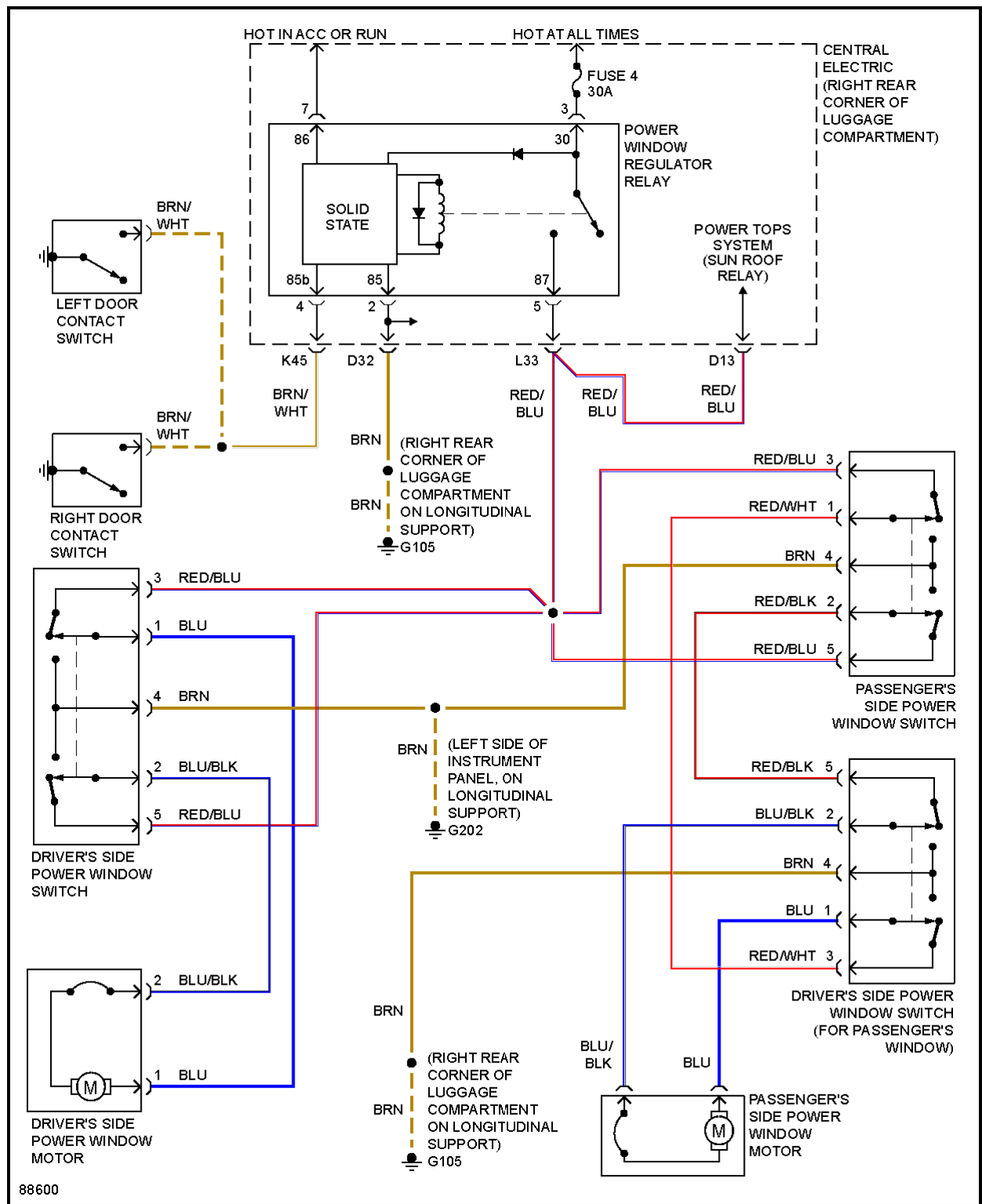
Fig. 8: Power Window Circuit
