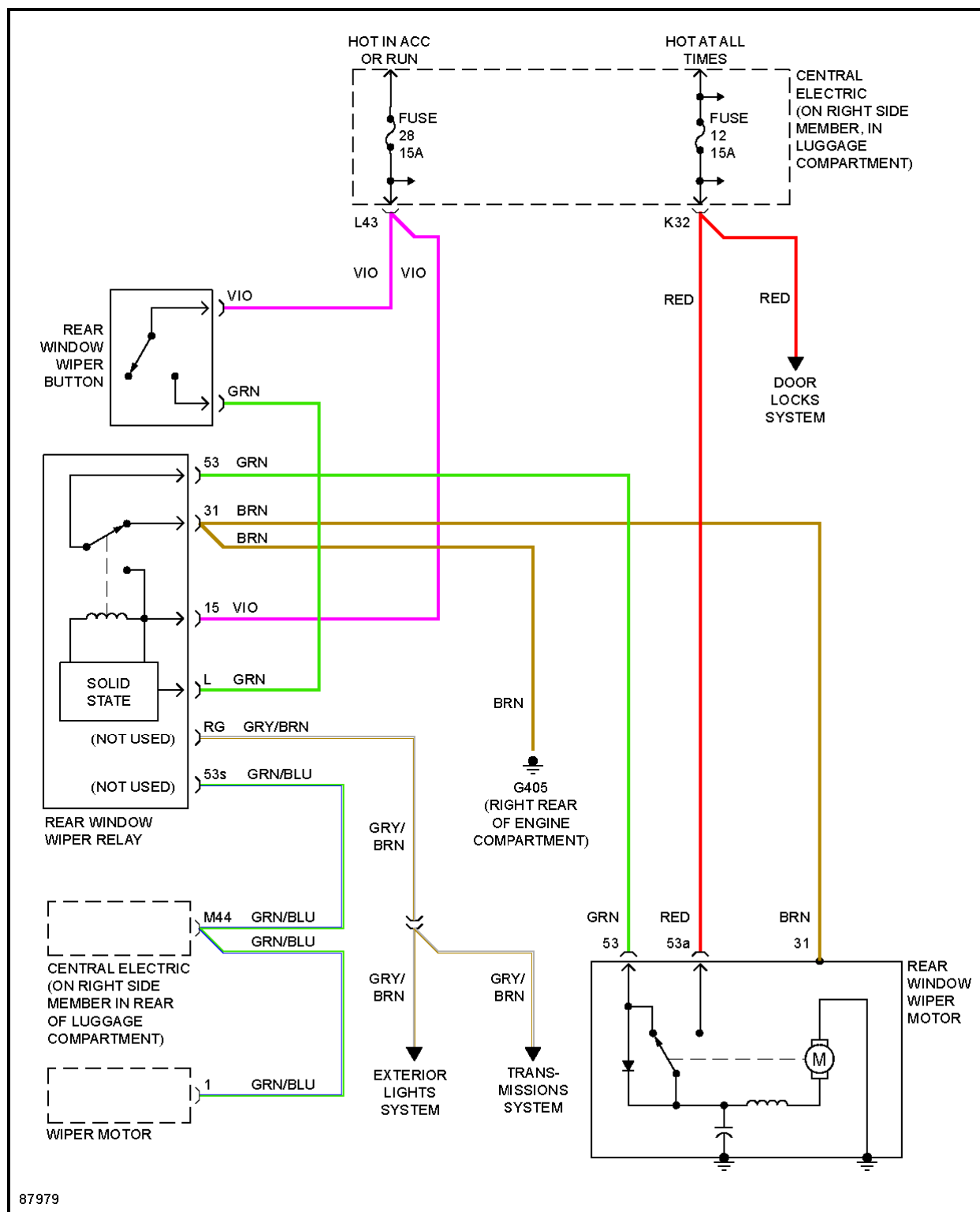
Fig. 14: Rear Wiper Circuit
