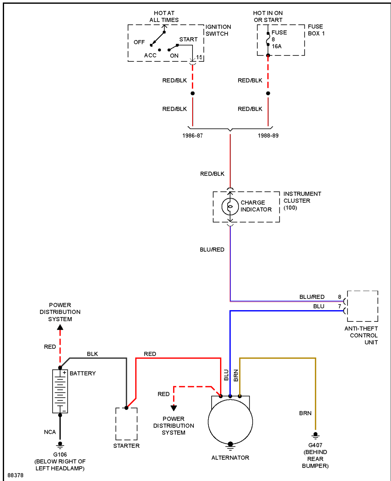
Fig. 11: Charging Circuit
