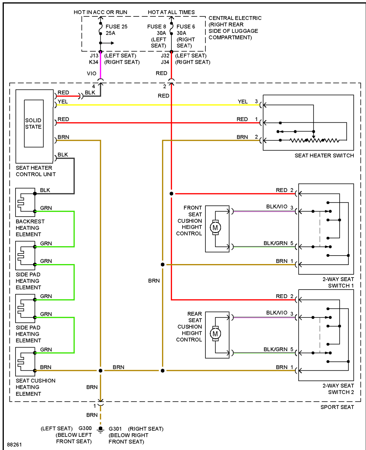
Fig. 7: Sport Seats Circuit
