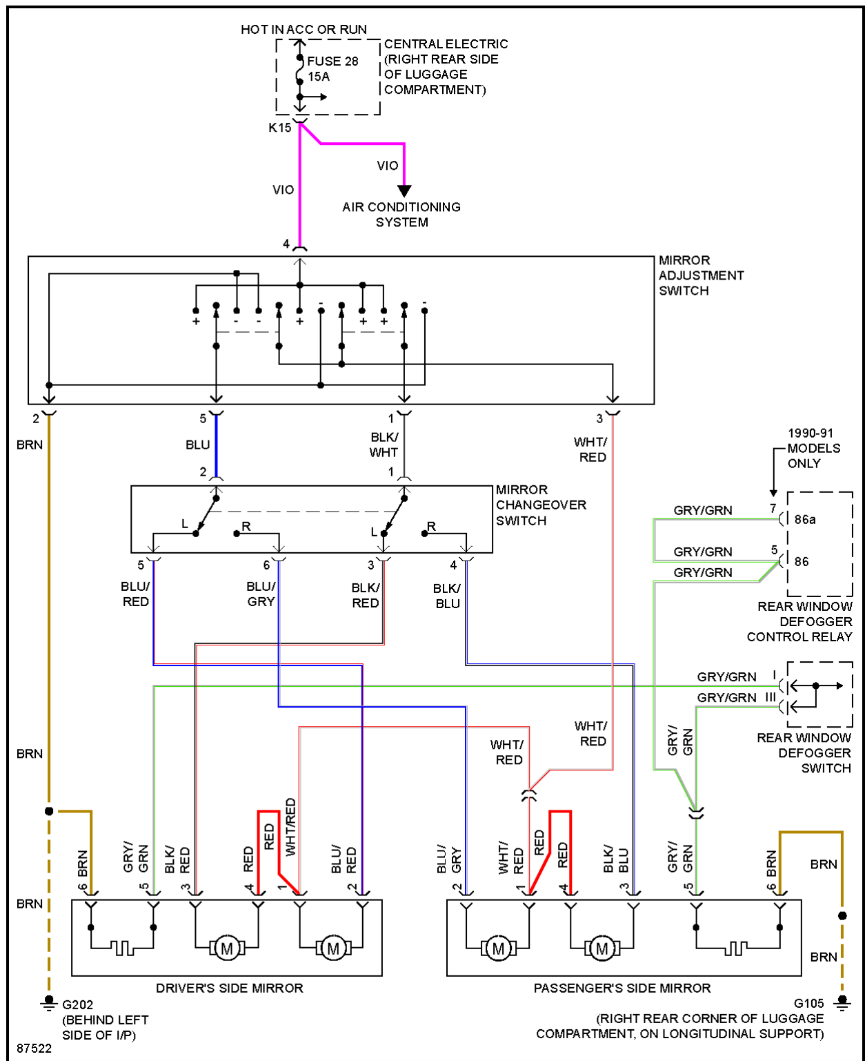
Fig. 5: Power Mirror Circuit
