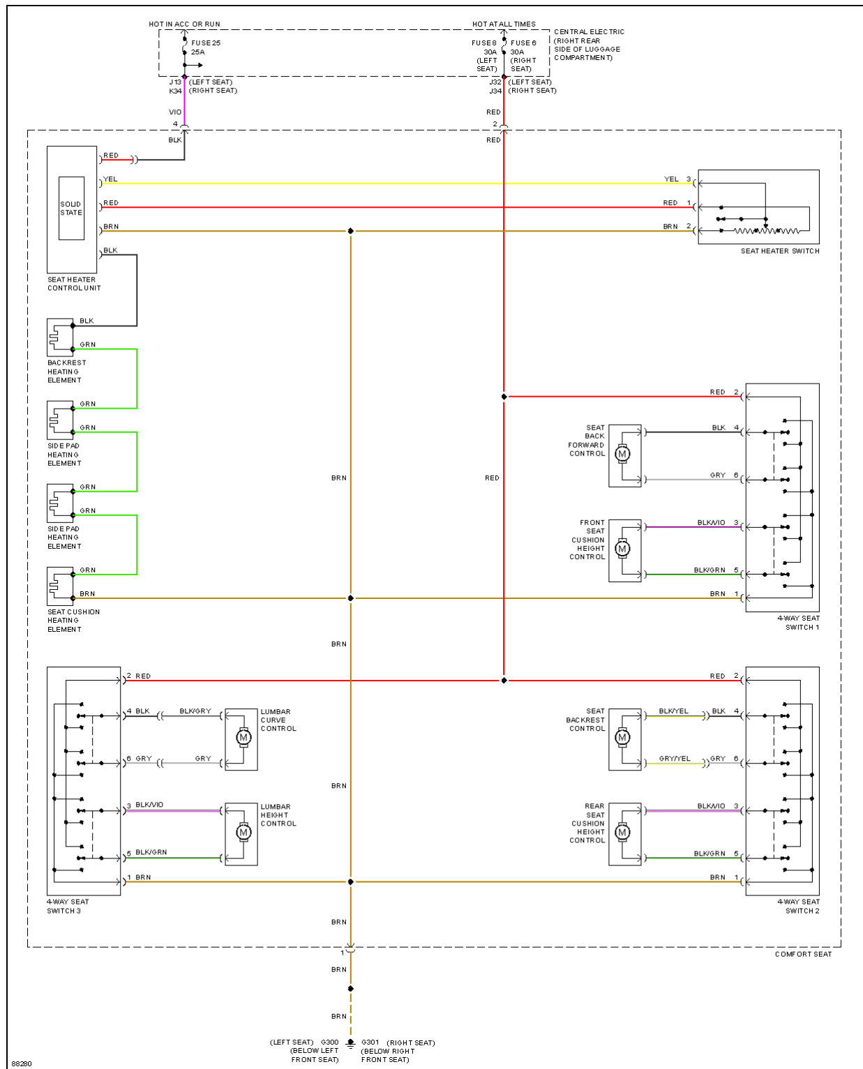
Fig. 6: Comfort Seats Circuit
